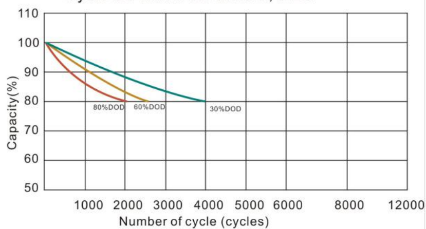
Cycle life with DOD at 25°C, 0.2C
