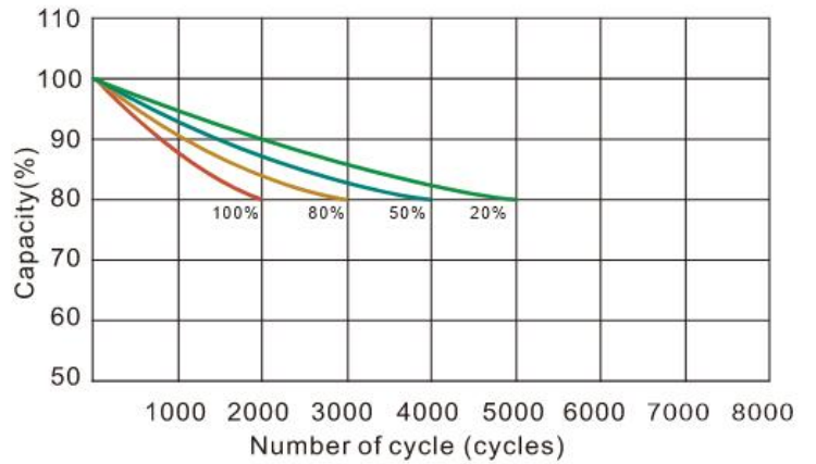
Cycle life with DOD at 25°C, 0.5C
